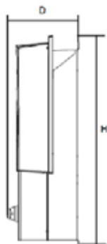
Wall Mount (PX12-1 - PX12-4)
